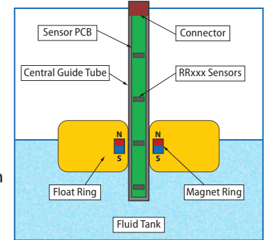
Figure 3. Magnet embedded in plastic float for use in fluid level sensing
